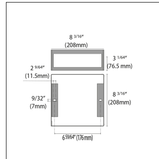
Facade Cover
